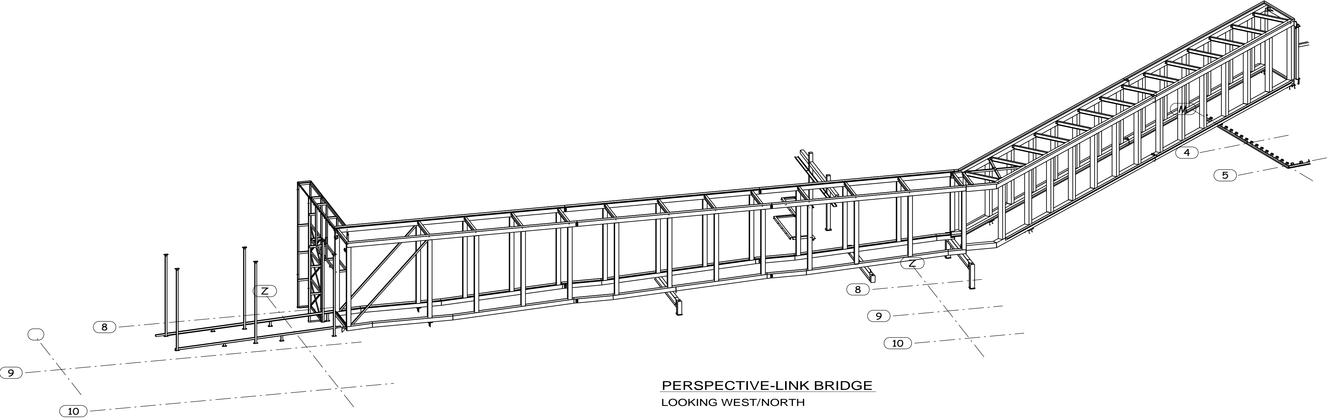
PERSPECTIVE-MAIN BUILDING LOOKING WEST/NORTH TOTAL WEIGHT: 121.3 MTON
