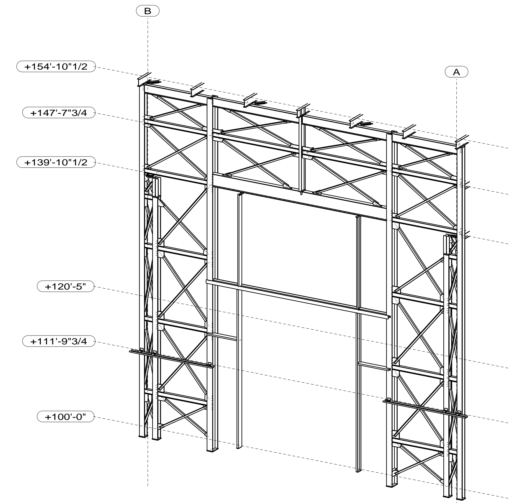
PERSPECTIVE ELEVATION LINE 1
