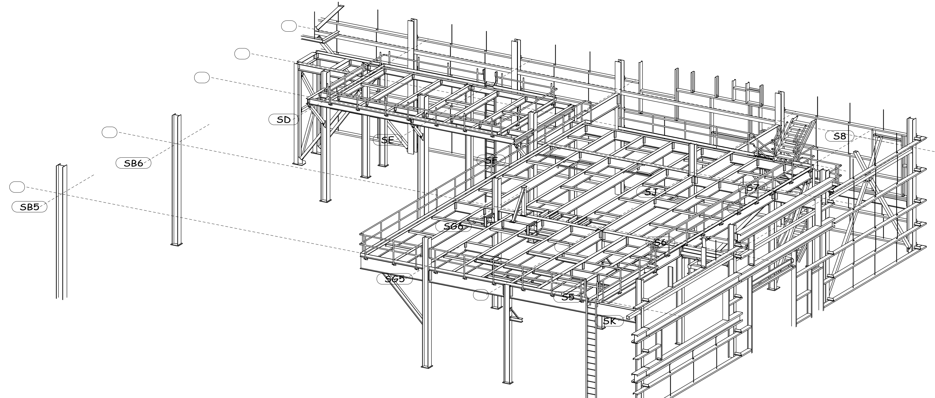
PERSPECTIVE-MEZZ. LOOKING NORTH/WEST
