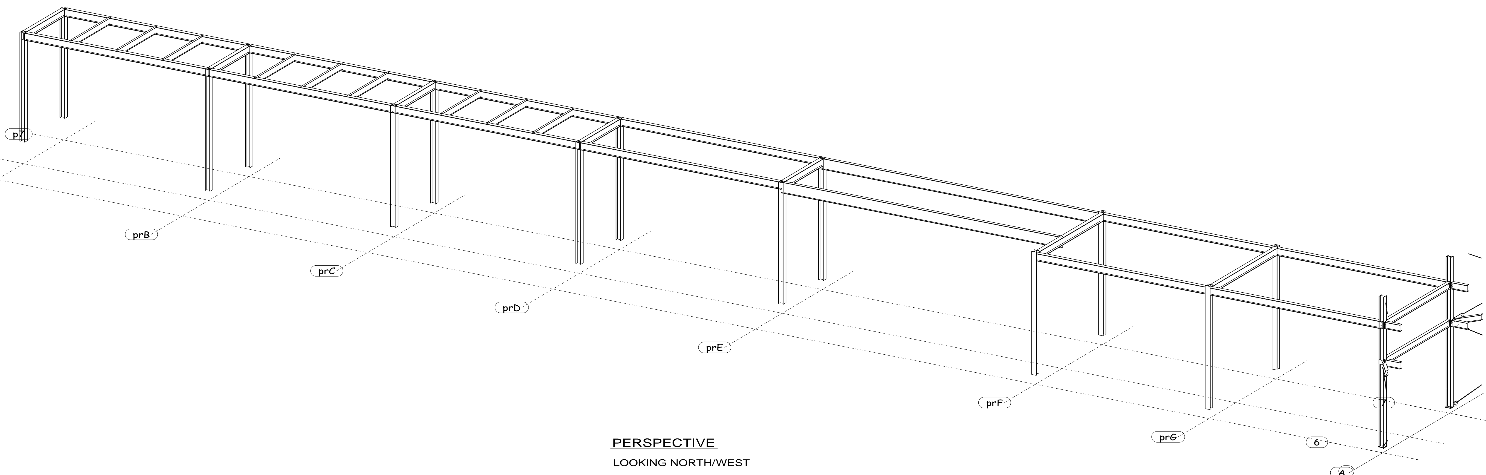
PERSPECTIVE LOOKING NORTH/WEST WEIGHT: 205.9 MTON
